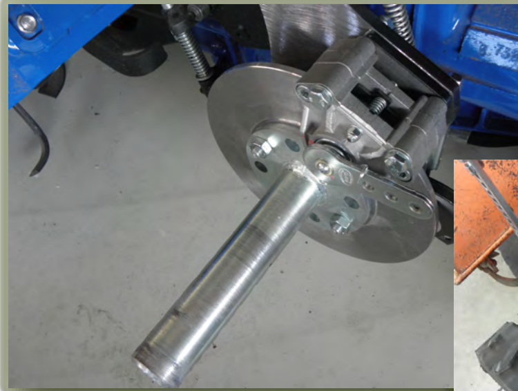
DISC BRAKE KIT APPLICABLE TO ALL VERSIONS
